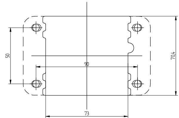
Reccomended firewall cutout
